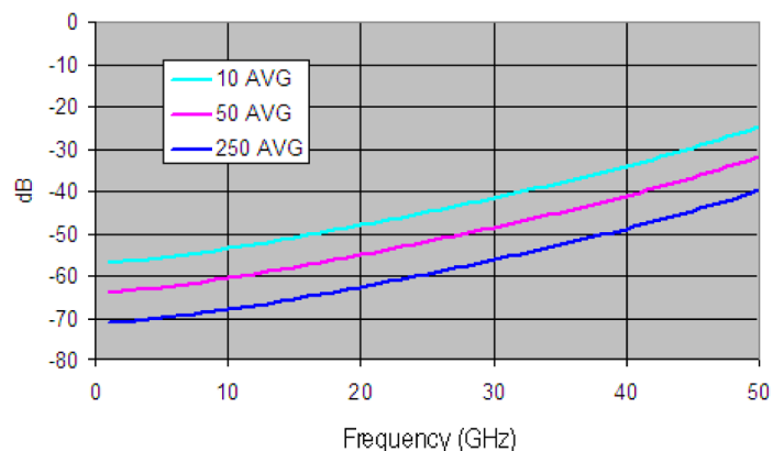
80E10B Insertion Loss (S21) Dynamic Range
